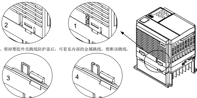
图 7-9 MD310T0.4B、MD310T0.7B、MD310T1.5B、MD310T2.2B、MD310T3.7B、MD310T5.5B 安规电容跳线位置及断开方法
